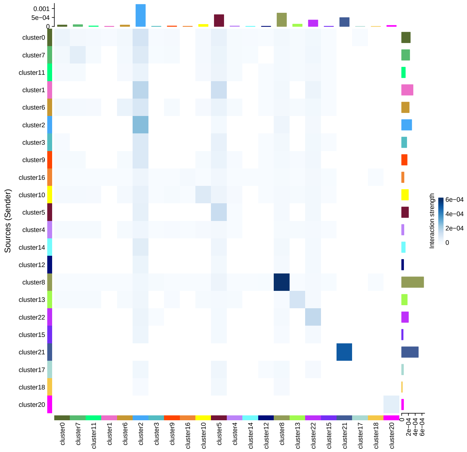
Interaction strength
